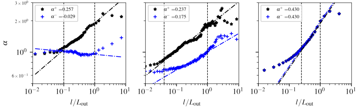
Figure 2. Exponential decrements of extended tails \alpha_l for \delta z_l^+ (black) and \delta z_l^- (blue) in fast solar wind (left), slow solar wind (center) and simulation (right). Here l/L_{\text{out}} represents the increment scale normalized with respect to the outer scale L_{\text{out}} which correspond to 700 s for fast wind, 2000 s for slow wind and 256\delta x for simulations. Vertical lines represents the limits of the inertial range.
