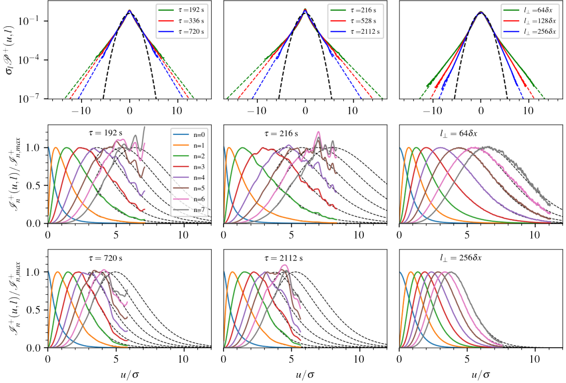
Figure 1. Top panels: continuous lines represent the estimated Probability Distribution Functions \mathcal{P}^+(u, l) versus u/\sigma_l for fast wind (left), slow wind (middle) and simulation (right), where u = \delta z_L^+ . Note that for spacecraft data the space lag is l = V_{sw} \tau via Taylor's Hypothesis, and \sigma_l represents the standard deviation at scale l . Middle and bottom panels: distribution of n^{\text{th}} moment \mathcal{S}_n^+(u, l) normalized to its maximum value ( \mathcal{S}_{n, \text{max}}^+ ) for fast wind (left), slow wind (middle) and simulation (right) for two different lags near the end (middle panel) and beginning (bottom panel) of the inertial range. Dashed lines represents the approximation of the PDF extending the tails assuming an exponential approximation.
